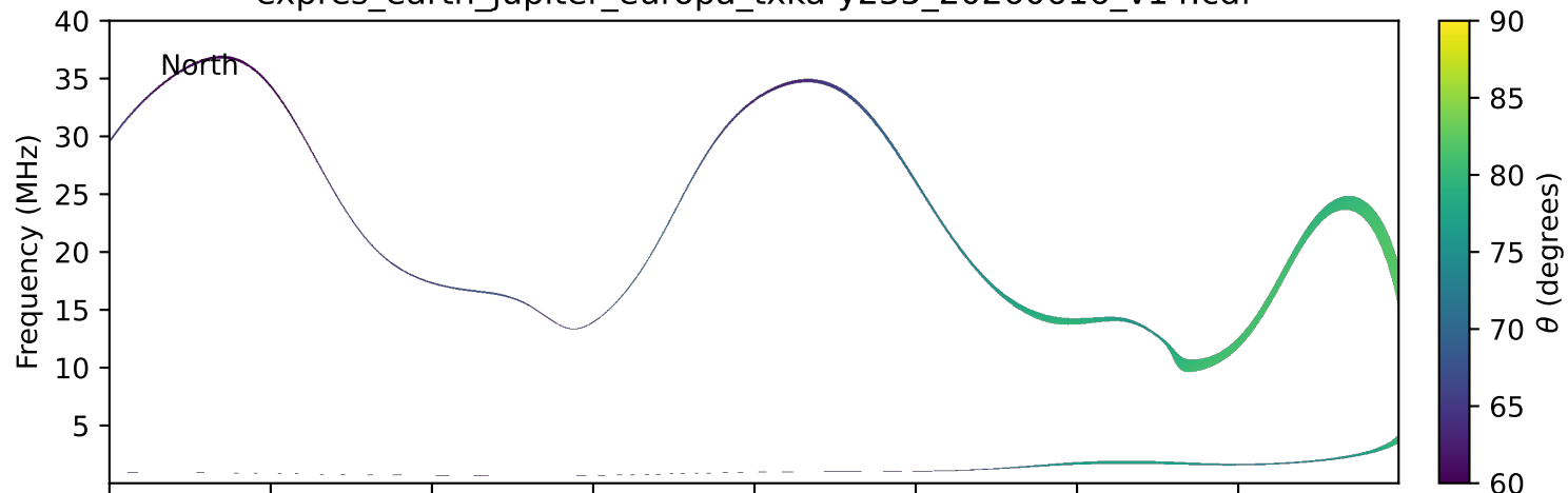
expres_earth_jupiter_europa_txka-y235_20260616_v14.cdf
