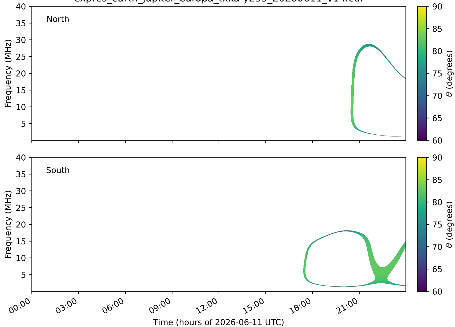
expres_earth_jupiter_europa_txka-y235_20260611_v14.cdf
