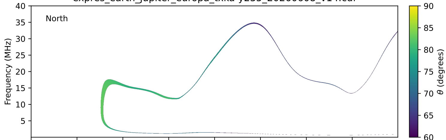
expres_earth_jupiter_europa_txka-y235_20260608_v14.cdf
