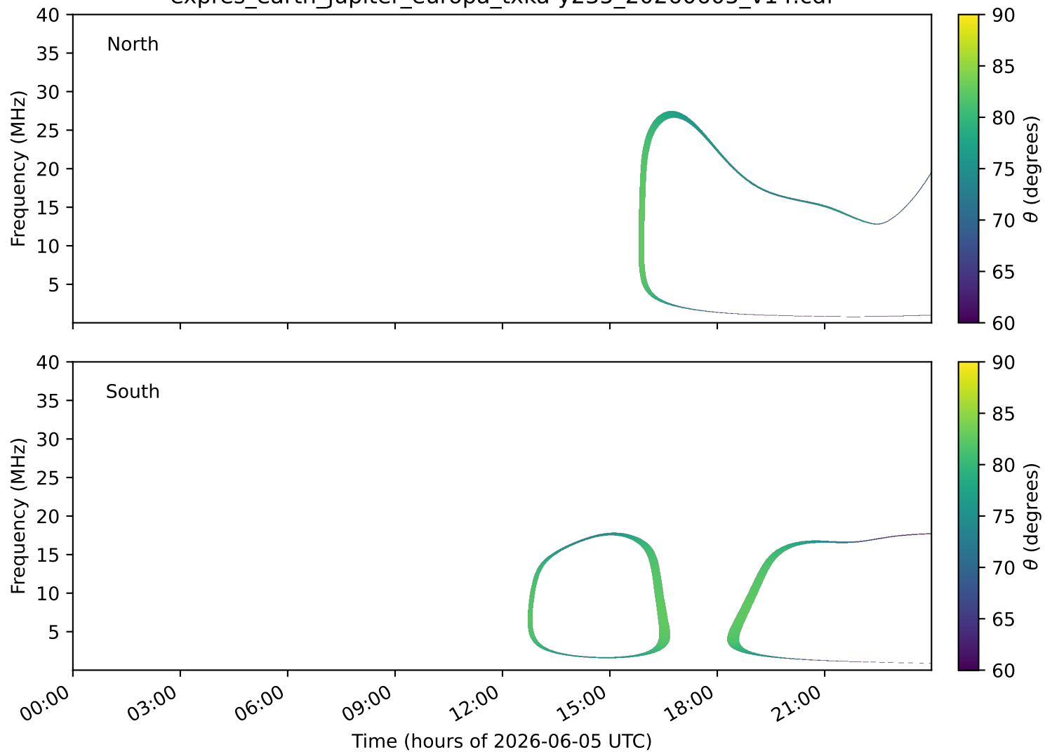
expres_earth_jupiter_europa_txka-y235_20260605_v14.cdf
