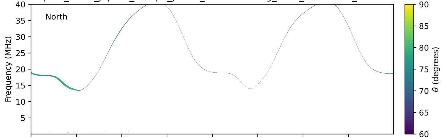
expres_earth_jupiter_europa_jrm33_lossc-wid1deg_3kev_20260612_v11.cdf
