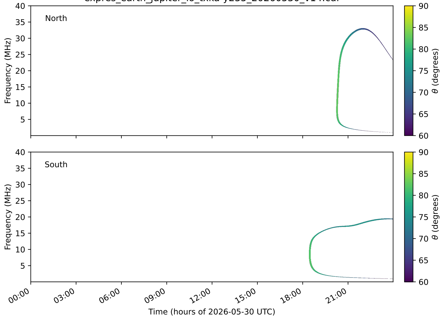
expres_earth_jupiter_io_txka-y235_20260530_v14.cdf
