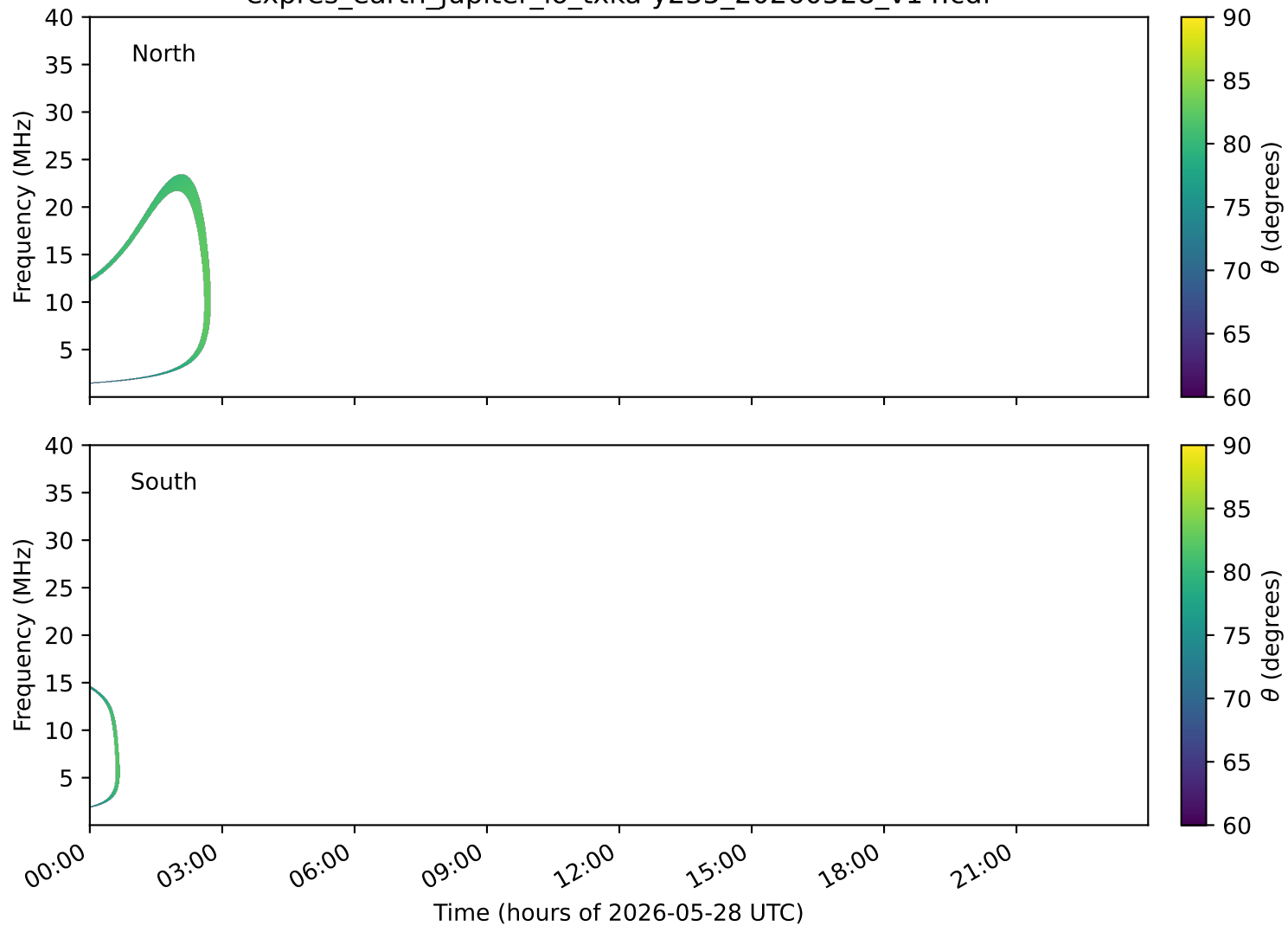
expres_earth_jupiter_io_txka-y235_20260528_v14.cdf
