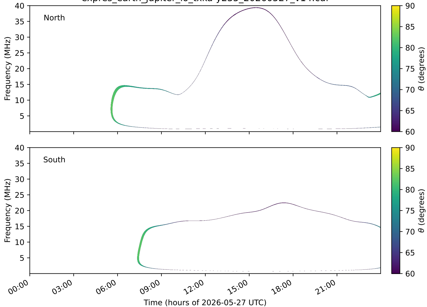
expres_earth_jupiter_io_txka-y235_20260527_v14.cdf
