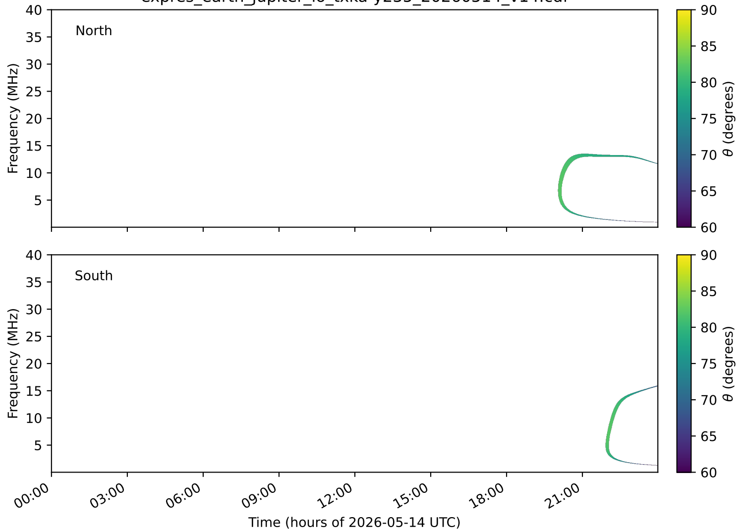
expres_earth_jupiter_io_txka-y235_20260514_v14.cdf
