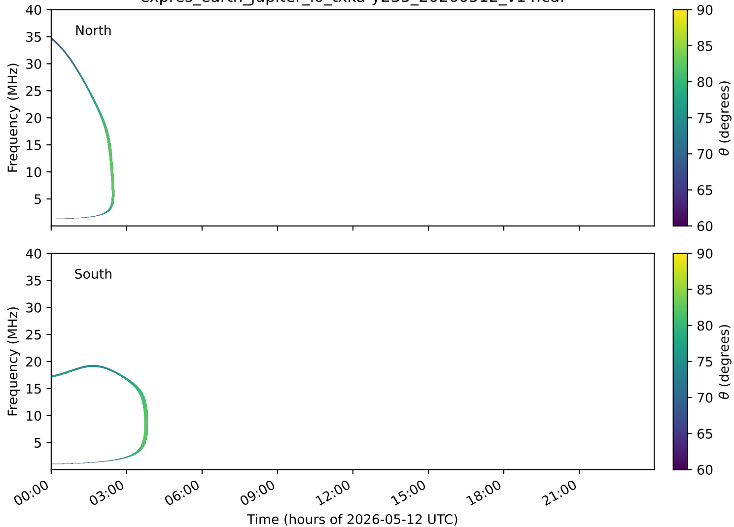
expres_earth_jupiter_io_txka-y235_20260512_v14.cdf
