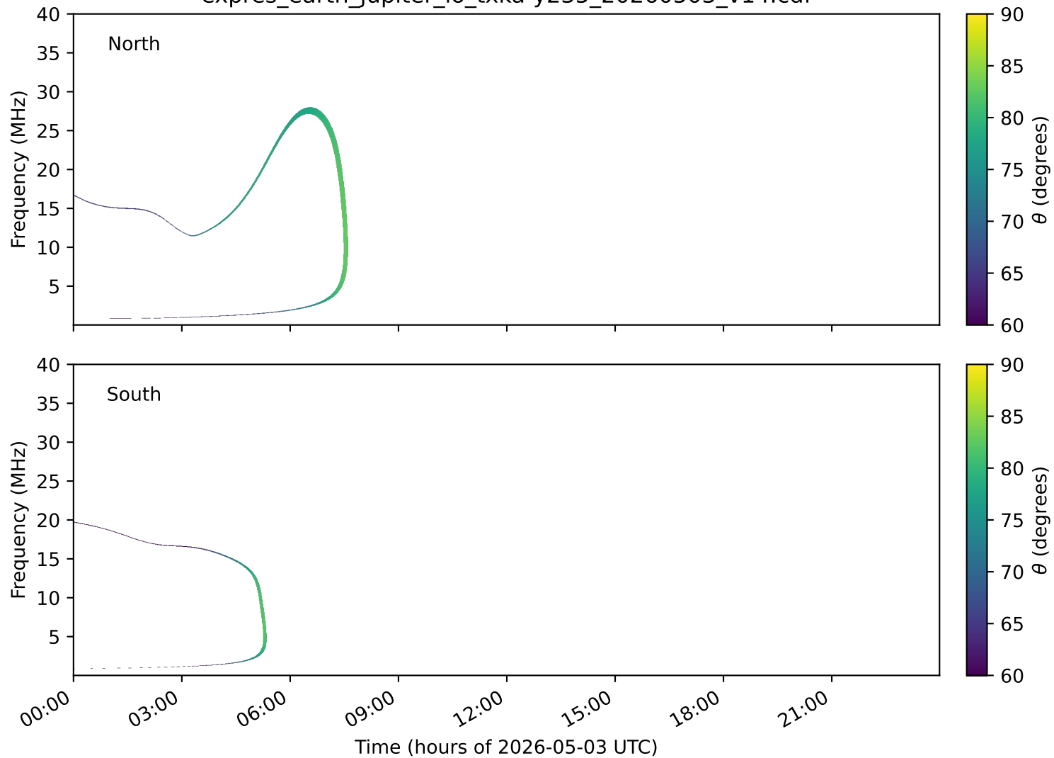
expres_earth_jupiter_io_txka-y235_20260503_v14.cdf
