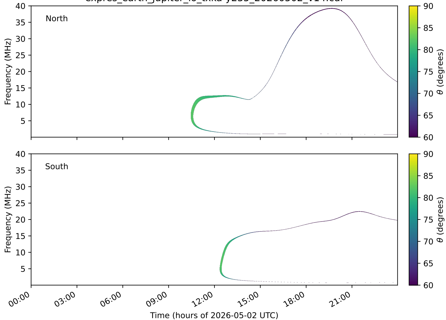
expres_earth_jupiter_io_txka-y235_20260502_v14.cdf
