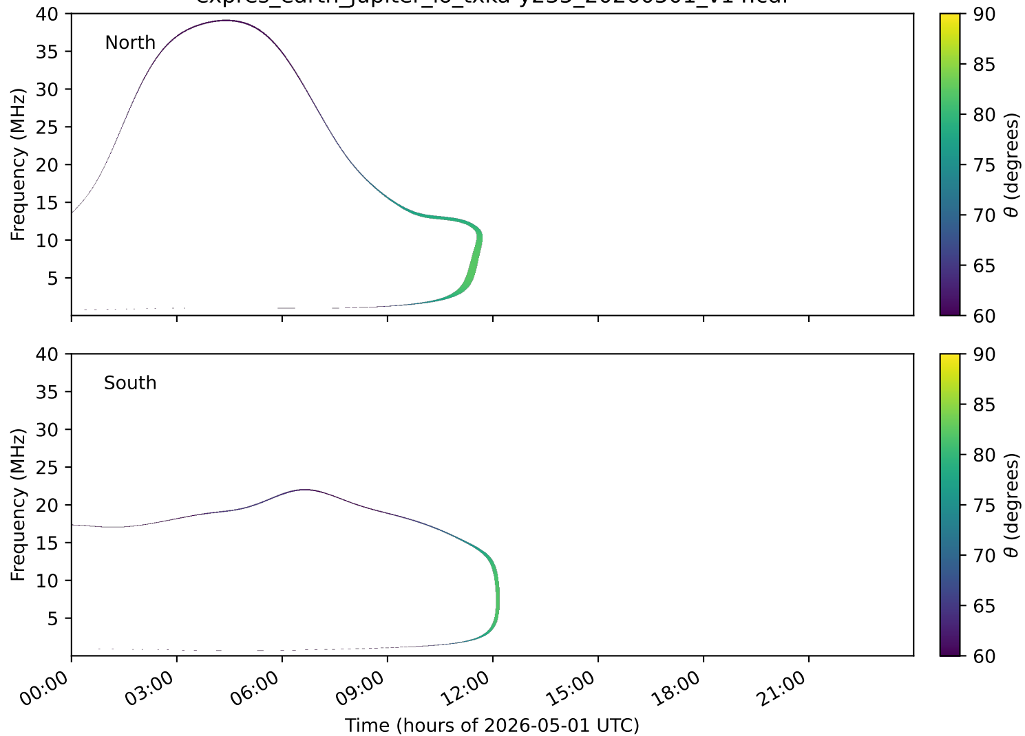
expres_earth_jupiter_io_txka-y235_20260501_v14.cdf
