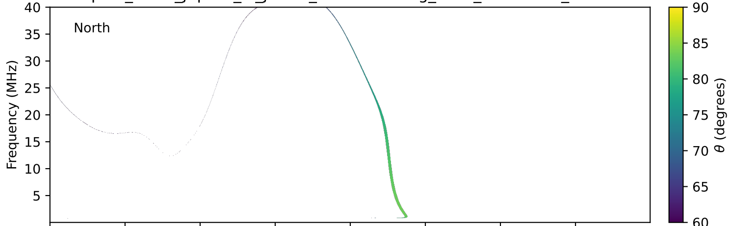
expres_earth_jupiter_io_jrm33_lossc-wid1deg_3kev_20260531_v11.cdf
