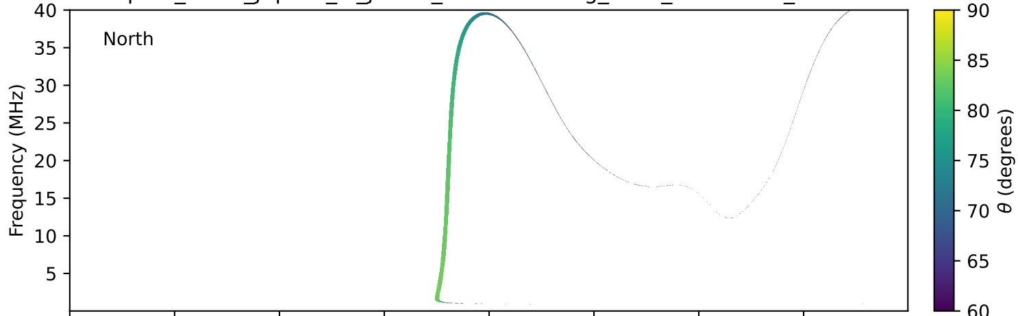
expres_earth_jupiter_io_jrm33_lossc-wid1deg_3kev_20260518_v11.cdf
