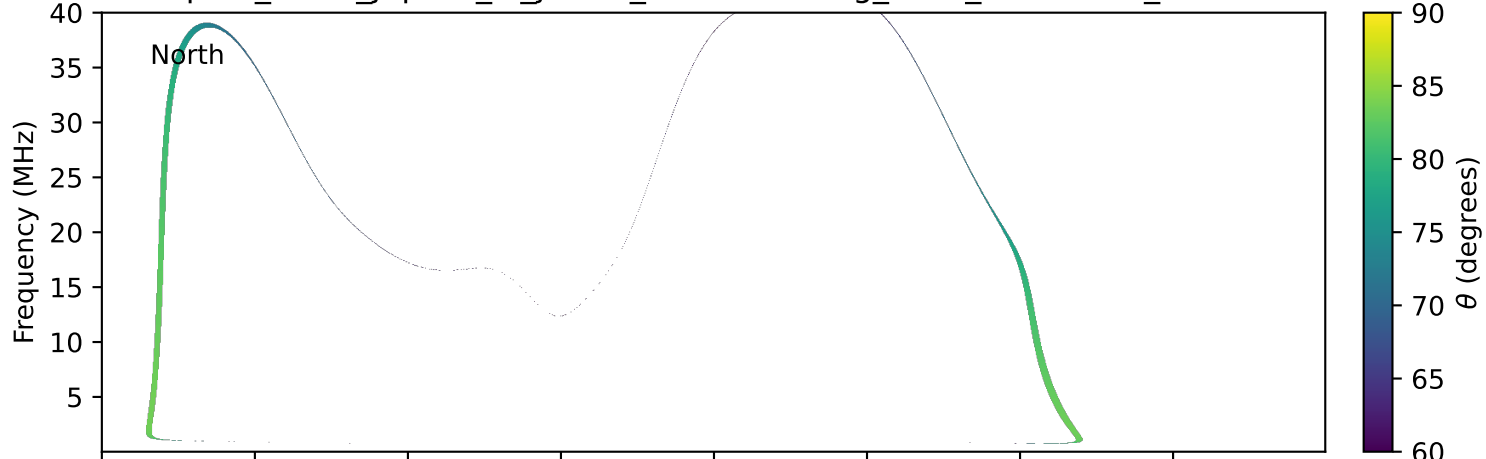
expres_earth_jupiter_io_jrm33_lossc-wid1deg_3kev_20260506_v11.cdf
