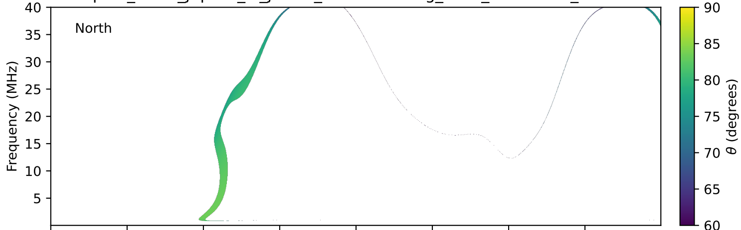
expres_earth_jupiter_io_jrm33_lossc-wid1deg_3kev_20260504_v11.cdf
