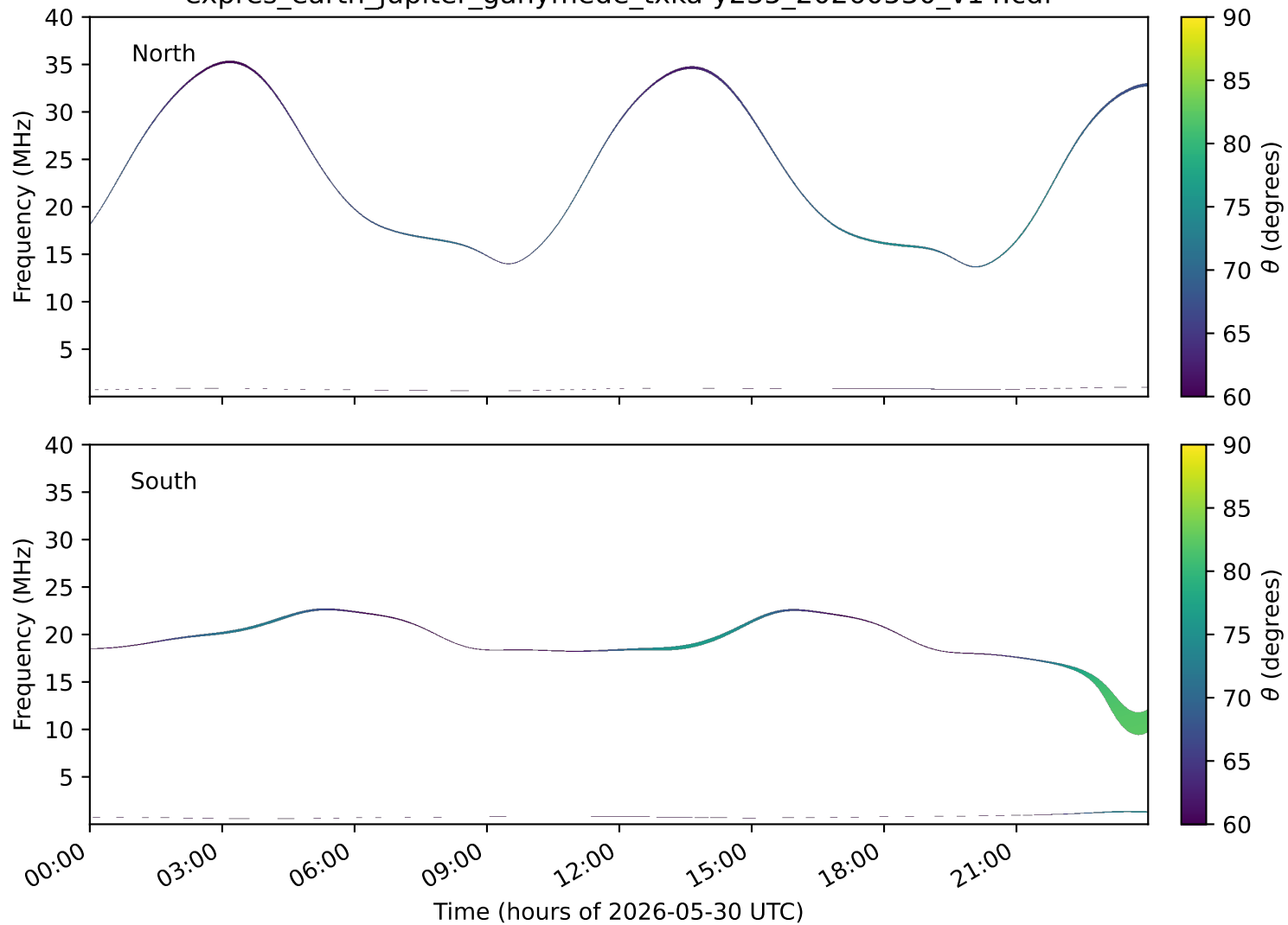
expres_earth_jupiter_ganymede_txka-y235_20260530_v14.cdf
