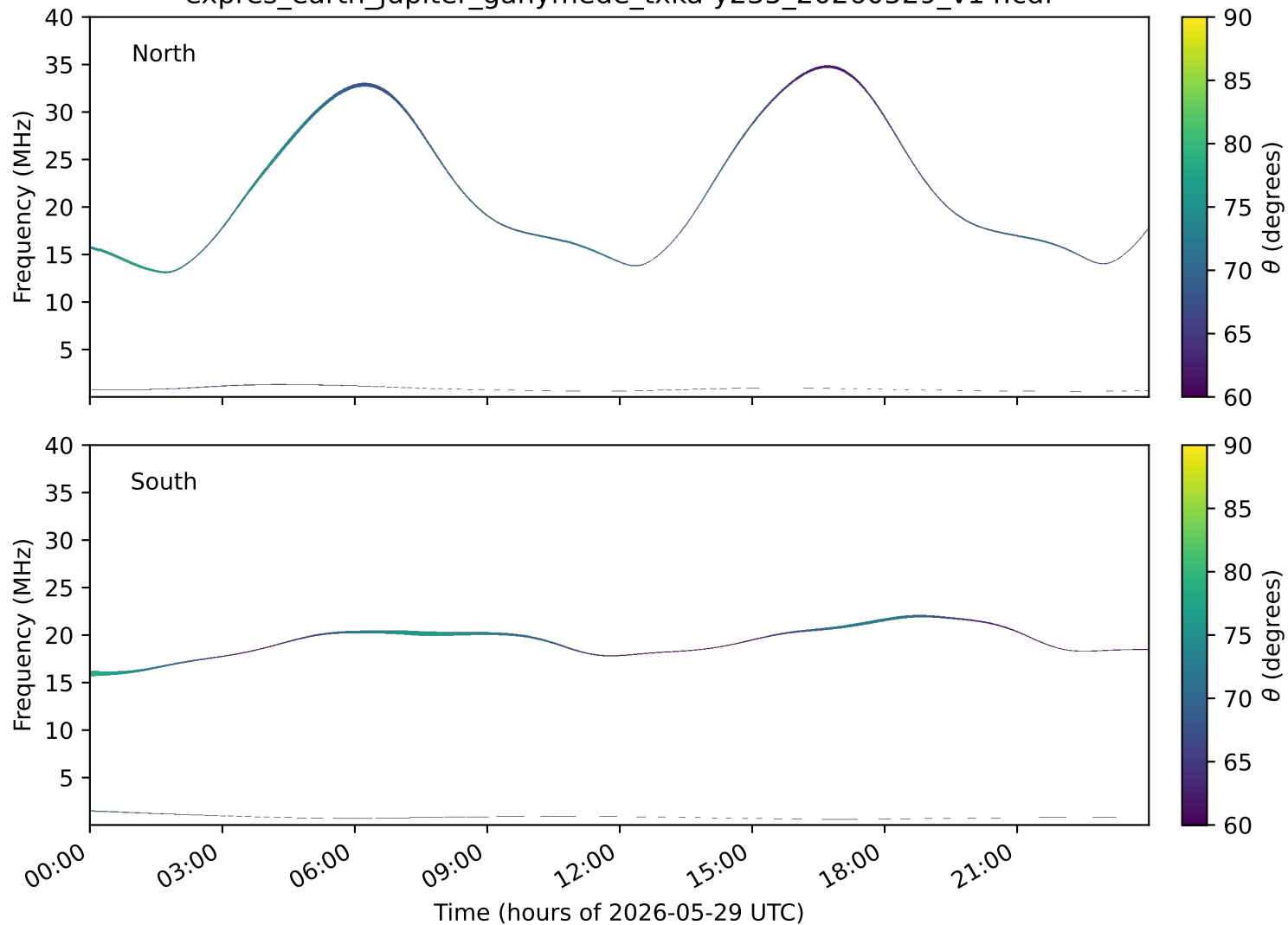
expres_earth_jupiter_ganymede_txka-y235_20260529_v14.cdf
