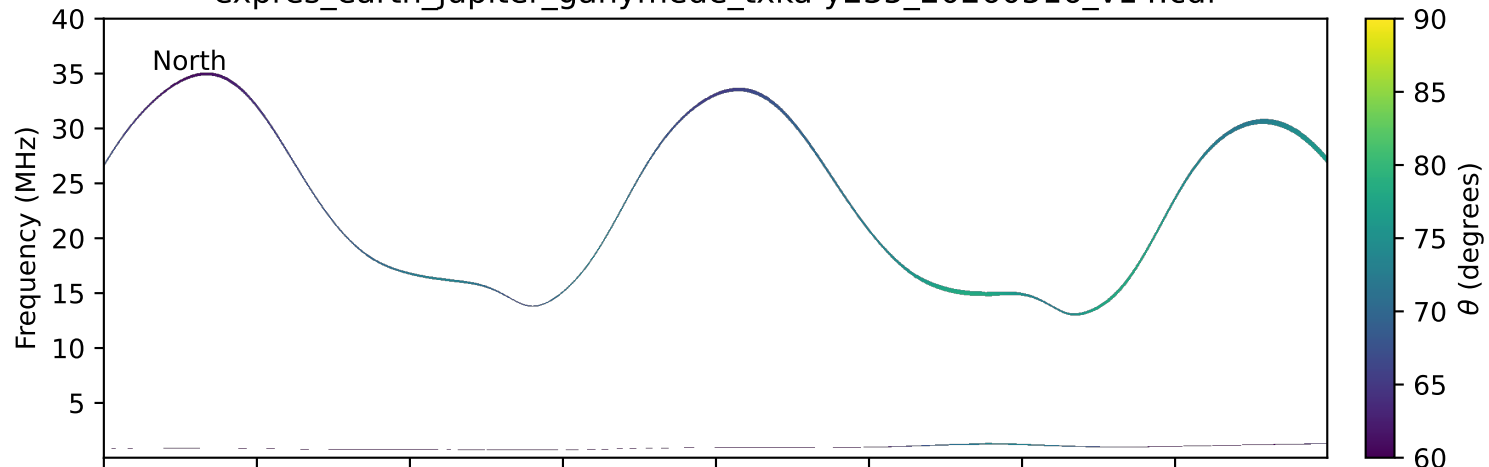
expres_earth_jupiter_ganymede_txka-y235_20260516_v14.cdf
