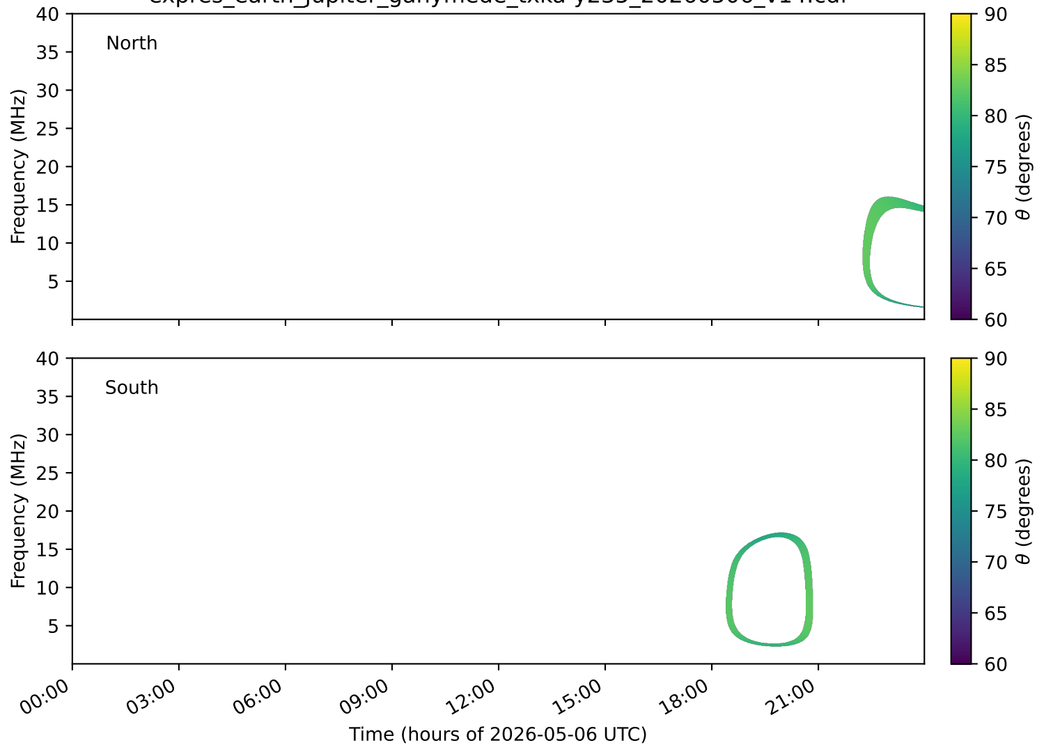
expres_earth_jupiter_ganymede_txka-y235_20260506_v14.cdf
