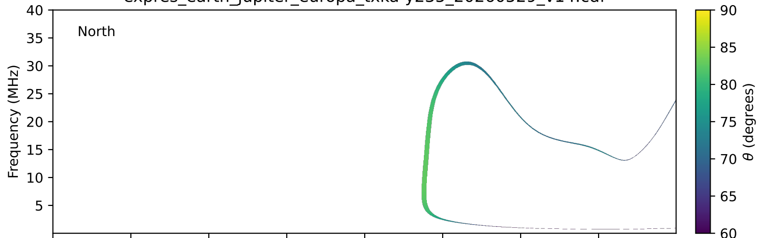
expres_earth_jupiter_europa_txka-y235_20260529_v14.cdf
