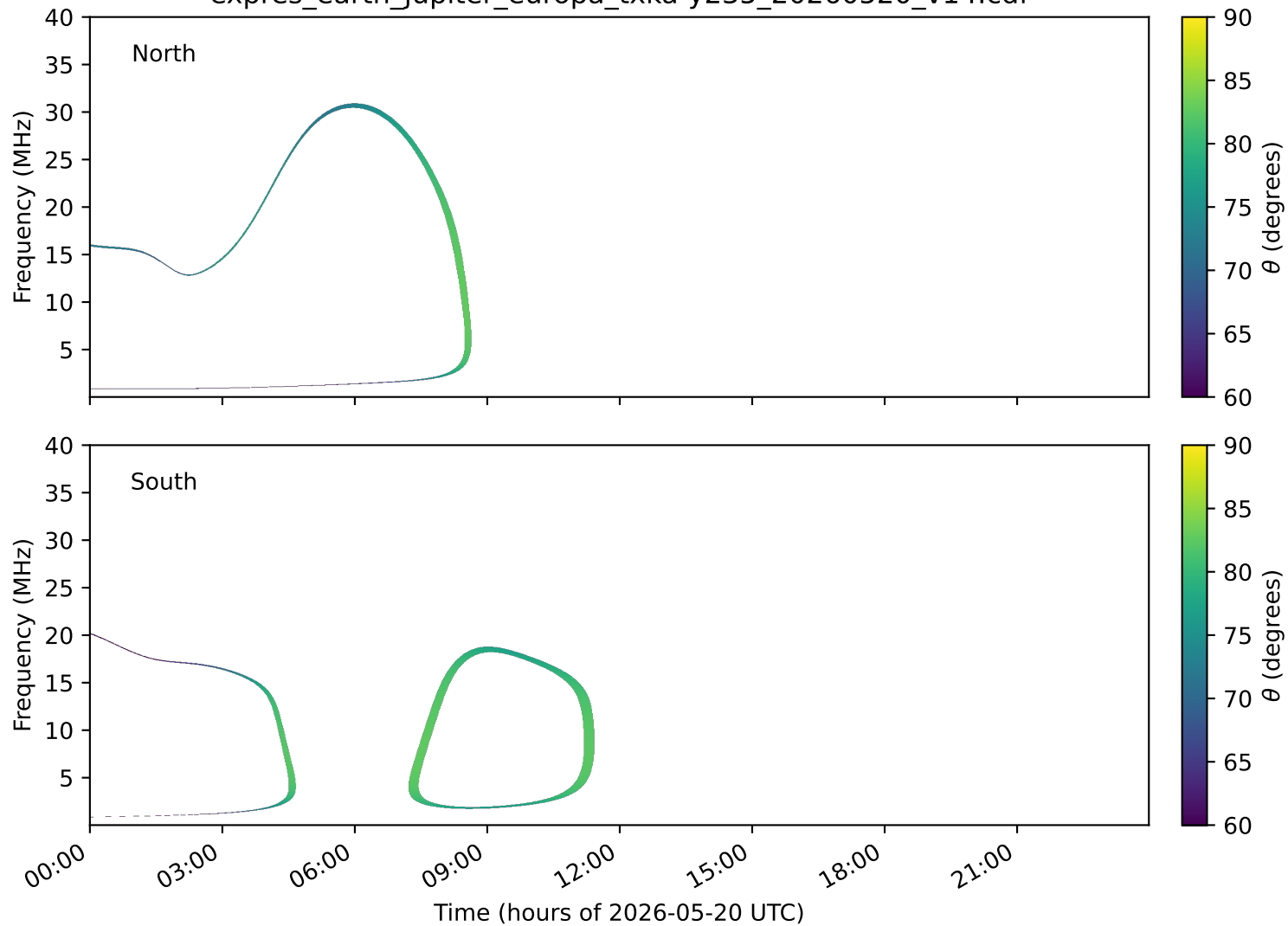
expres_earth_jupiter_europa_txka-y235_20260520_v14.cdf
