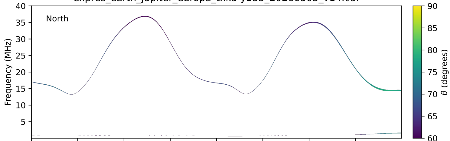
expres_earth_jupiter_europa_txka-y235_20260505_v14.cdf
