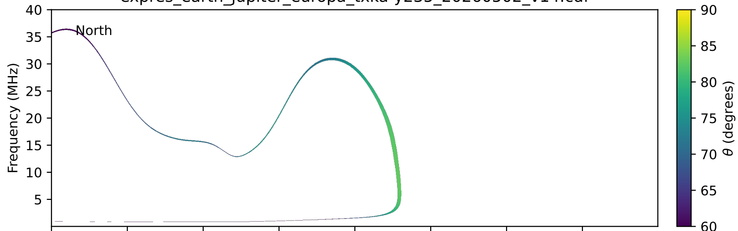
expres_earth_jupiter_europa_txka-y235_20260502_v14.cdf
