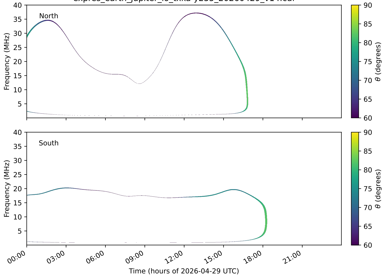
expres_earth_jupiter_io_txka-y235_20260429_v14.cdf
