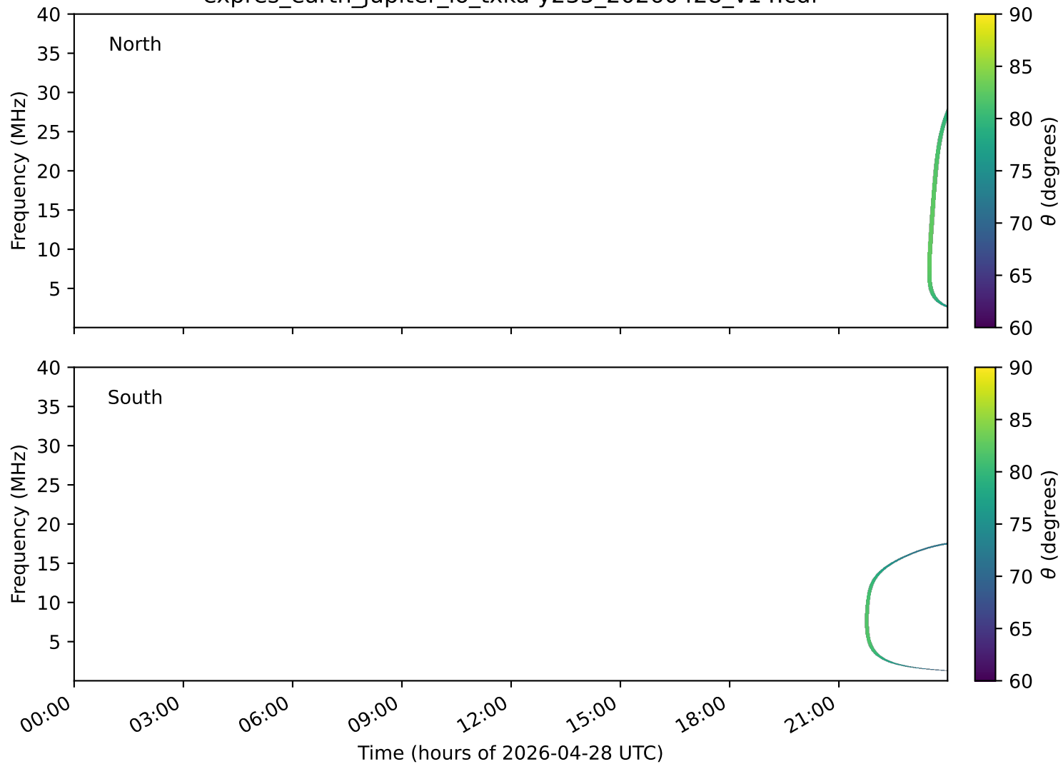
expres_earth_jupiter_io_txka-y235_20260428_v14.cdf
