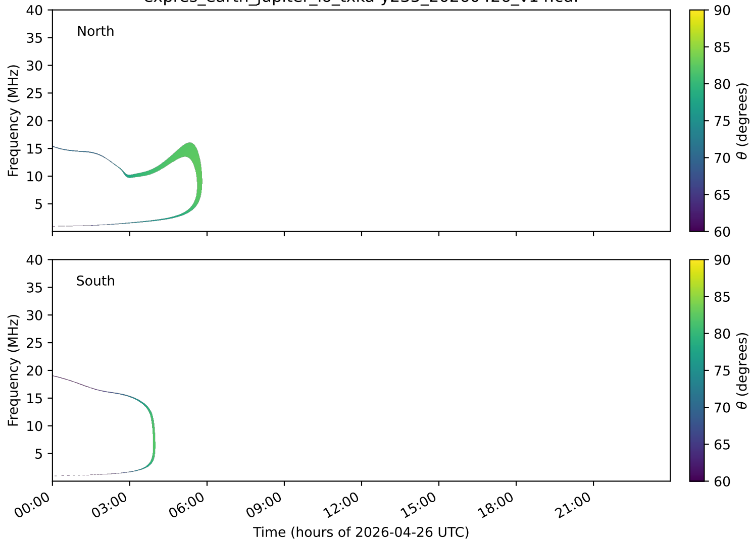
expres_earth_jupiter_io_txka-y235_20260426_v14.cdf
