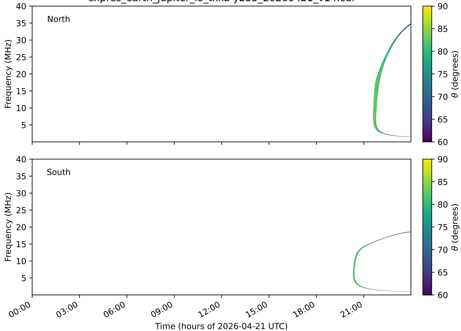
expres_earth_jupiter_io_txka-y235_20260421_v14.cdf
