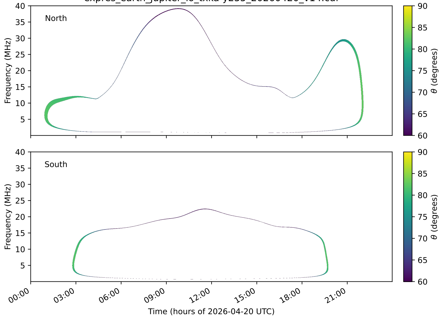
expres_earth_jupiter_io_txka-y235_20260420_v14.cdf
