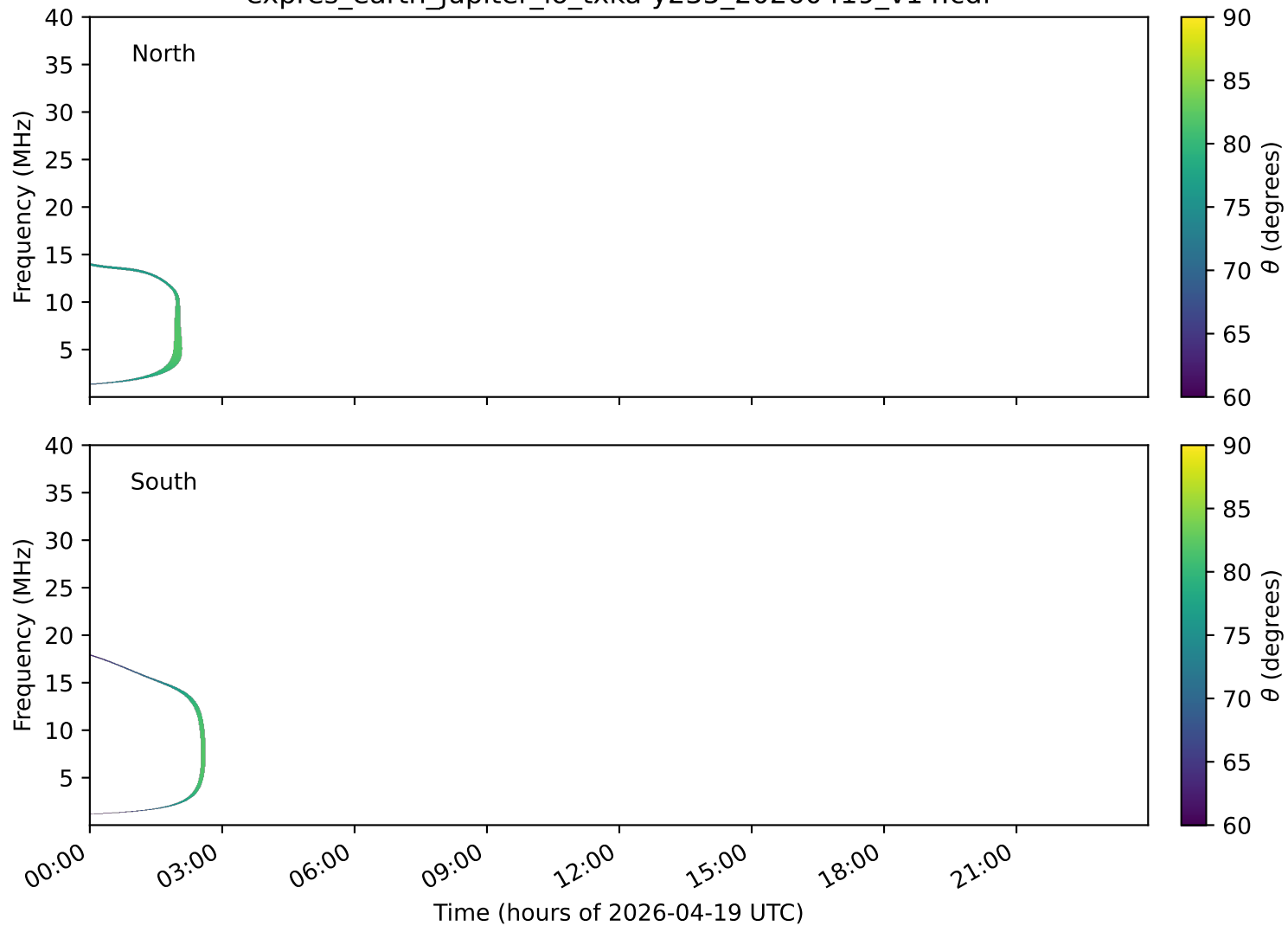
expres_earth_jupiter_io_txka-y235_20260419_v14.cdf
