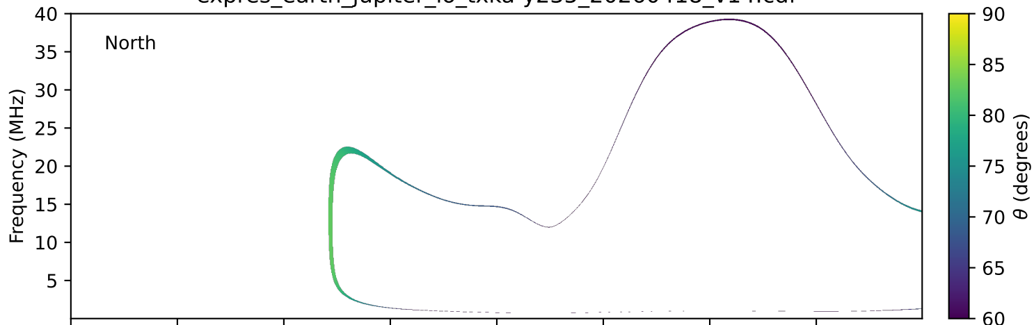
expres_earth_jupiter_io_txka-y235_20260418_v14.cdf
