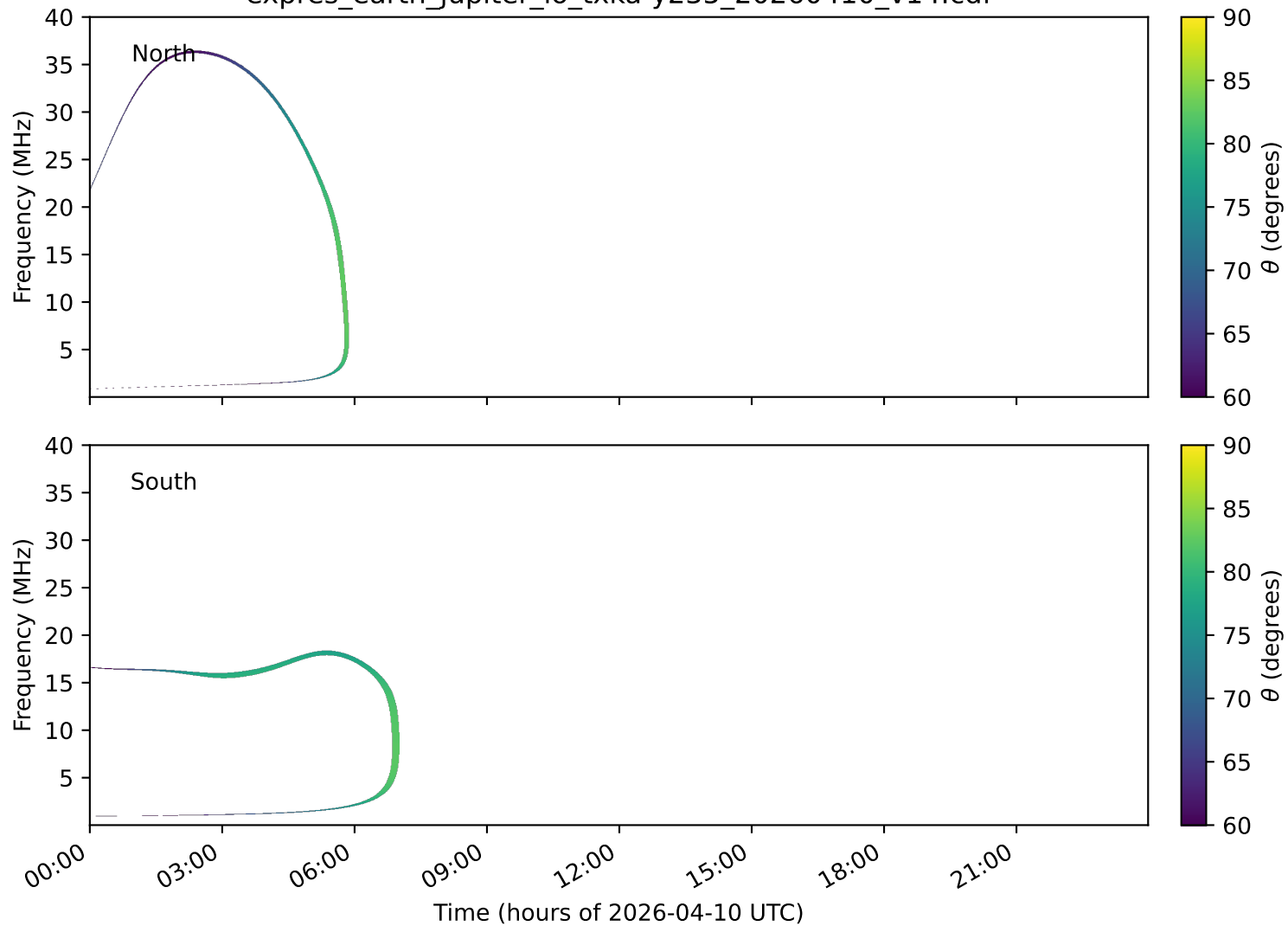
expres_earth_jupiter_io_txka-y235_20260410_v14.cdf
