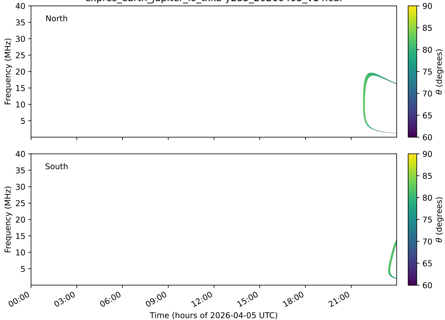
expres_earth_jupiter_io_txka-y235_20260405_v14.cdf
