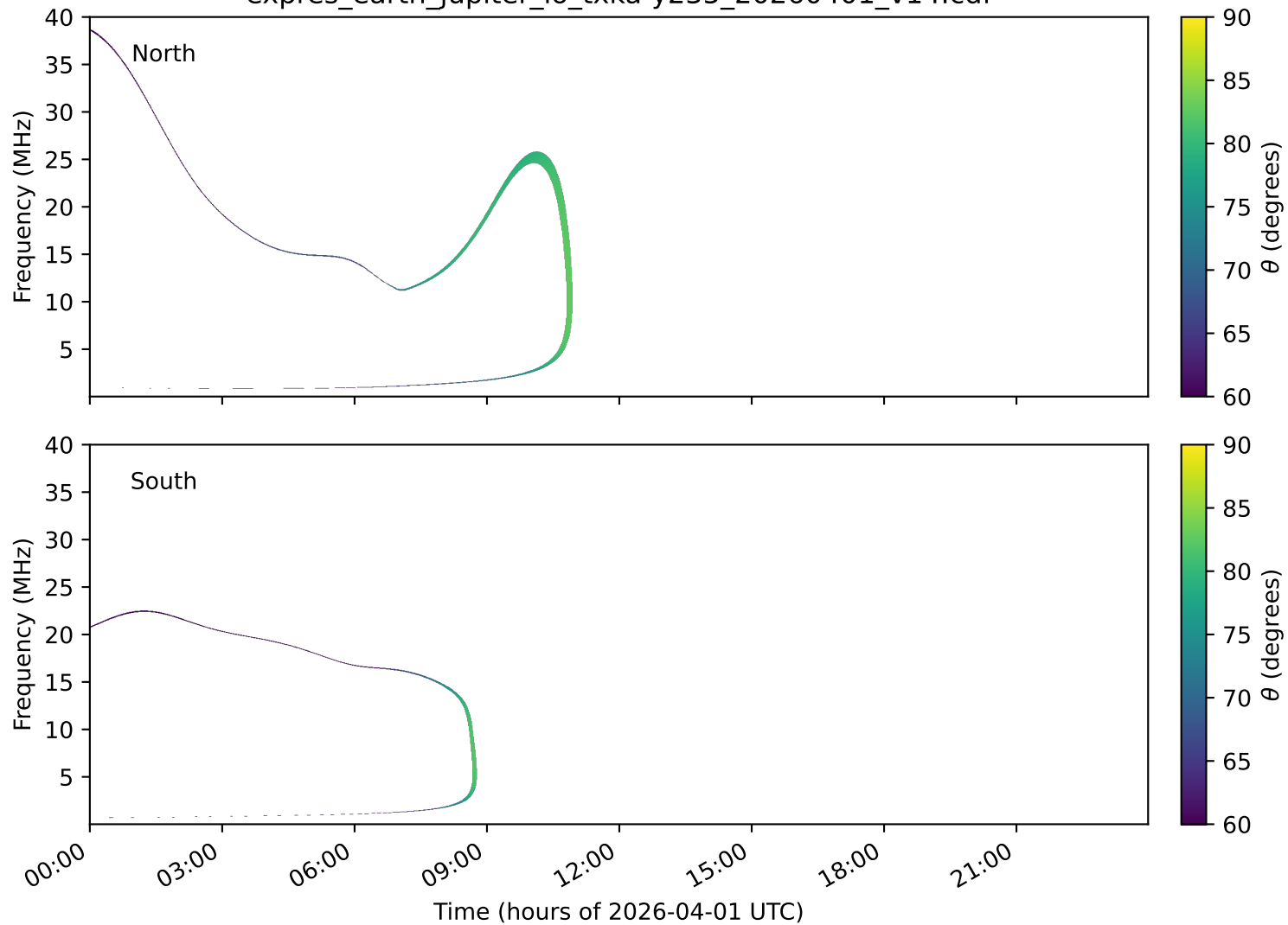
expres_earth_jupiter_io_txka-y235_20260401_v14.cdf
