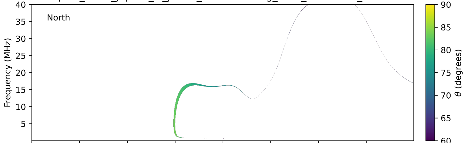
expres_earth_jupiter_io_jrm33_lossc-wid1deg_3kev_20260425_v11.cdf
