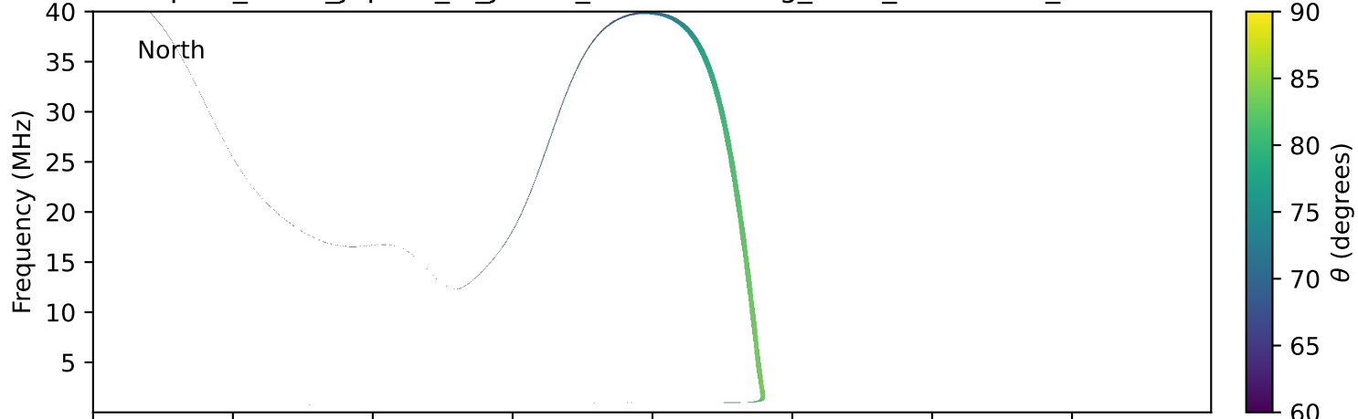
expres_earth_jupiter_io_jrm33_lossc-wid1deg_3kev_20260415_v11.cdf
