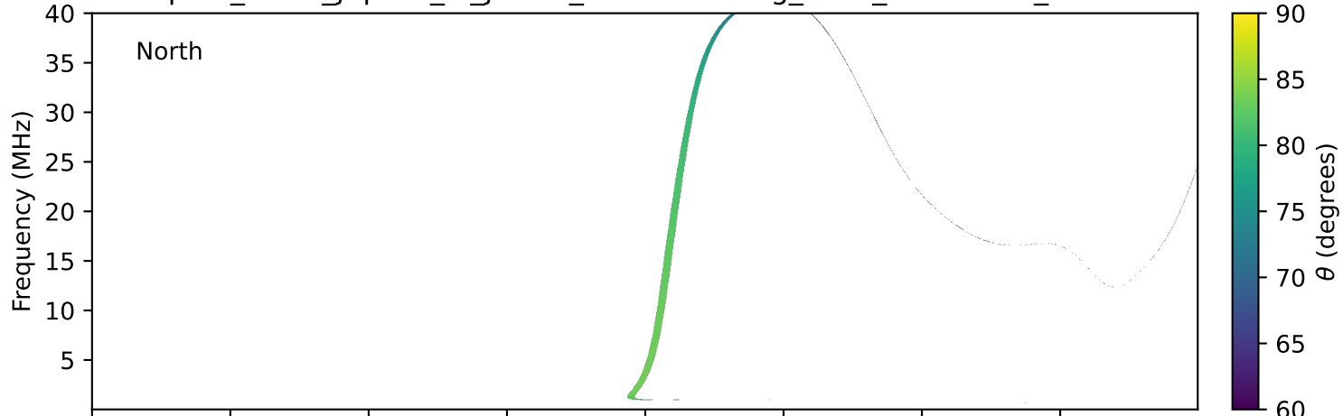
expres_earth_jupiter_io_jrm33_lossc-wid1deg_3kev_20260409_v11.cdf
