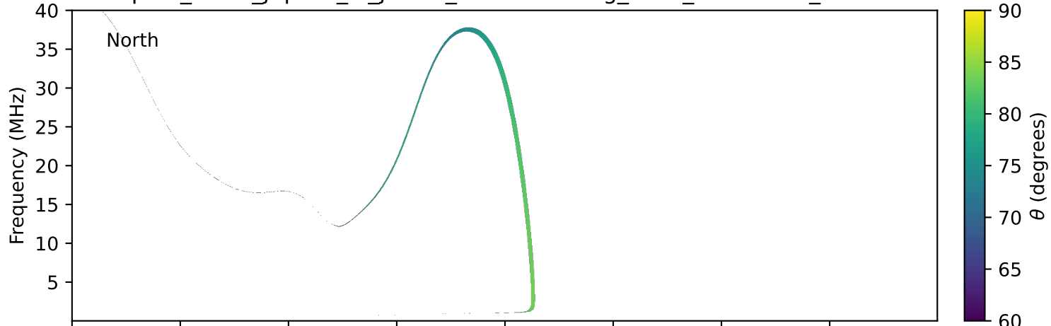
expres_earth_jupiter_io_jrm33_lossc-wid1deg_3kev_20260408_v11.cdf
