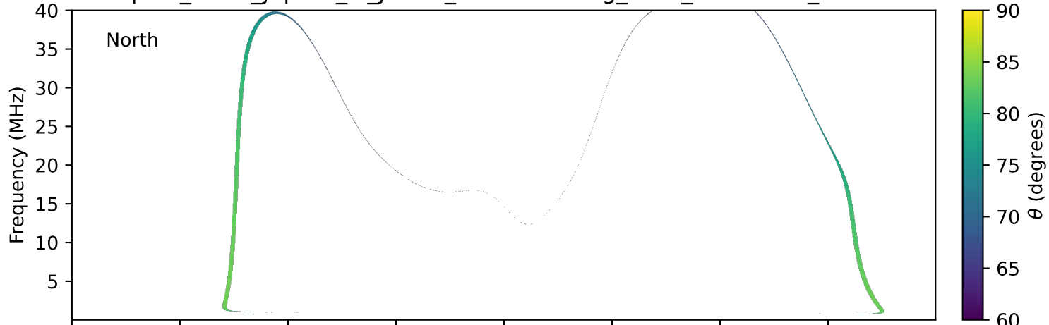
expres_earth_jupiter_io_jrm33_lossc-wid1deg_3kev_20260404_v11.cdf
