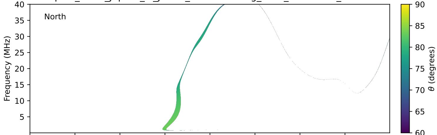
expres_earth_jupiter_io_jrm33_lossc-wid1deg_3kev_20260402_v11.cdf
