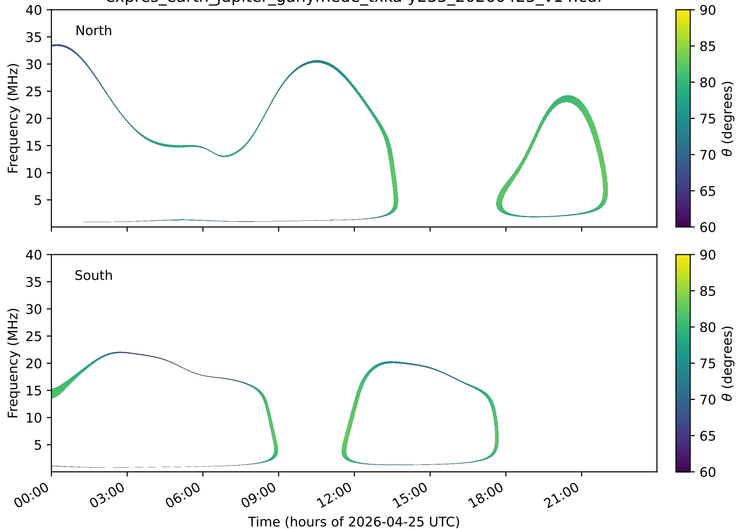
expres_earth_jupiter_ganymede_txka-y235_20260425_v14.cdf
