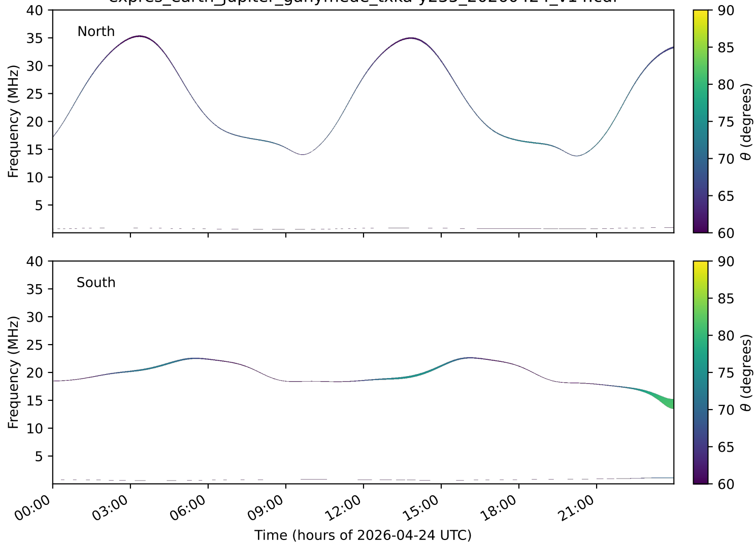
expres_earth_jupiter_ganymede_txka-y235_20260424_v14.cdf
