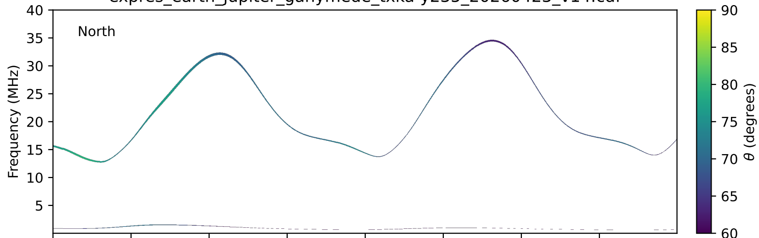
expres_earth_jupiter_ganymede_txka-y235_20260423_v14.cdf
