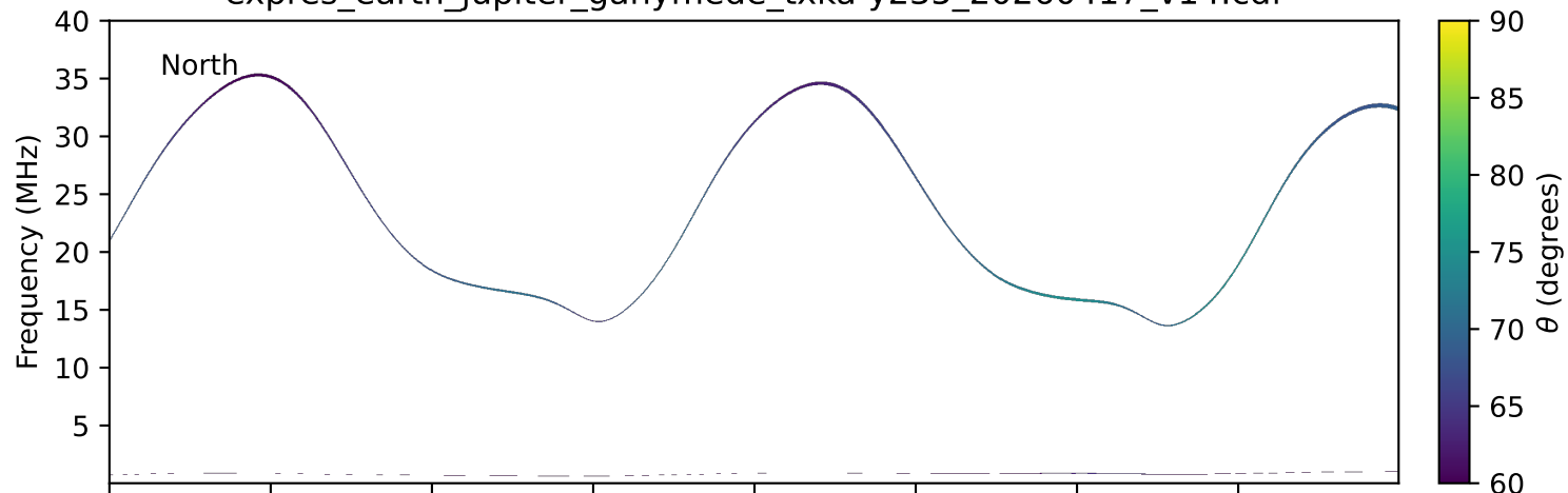
expres_earth_jupiter_ganymede_txka-y235_20260417_v14.cdf
