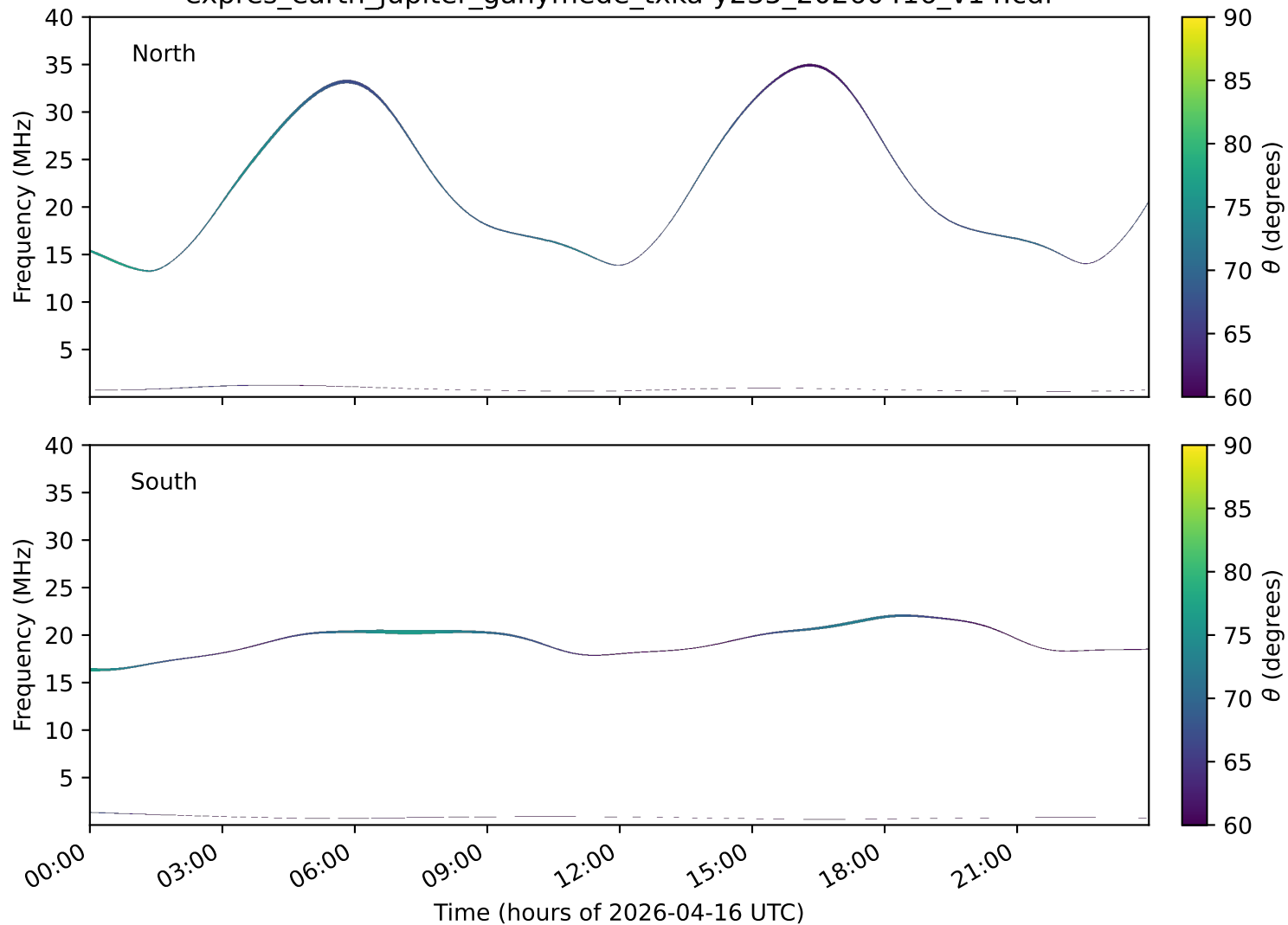
expres_earth_jupiter_ganymede_txka-y235_20260416_v14.cdf
