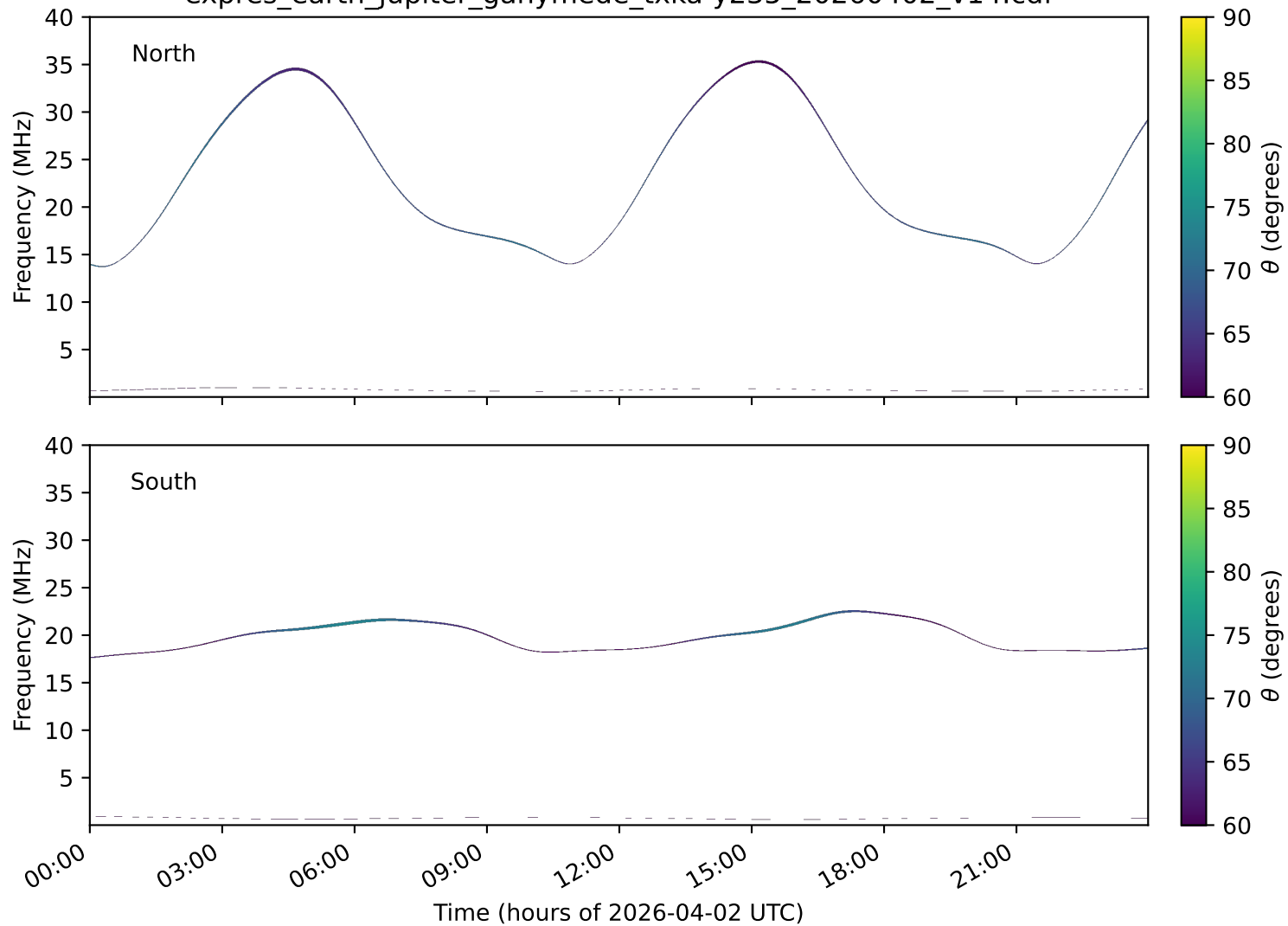
expres_earth_jupiter_ganymede_txka-y235_20260402_v14.cdf
