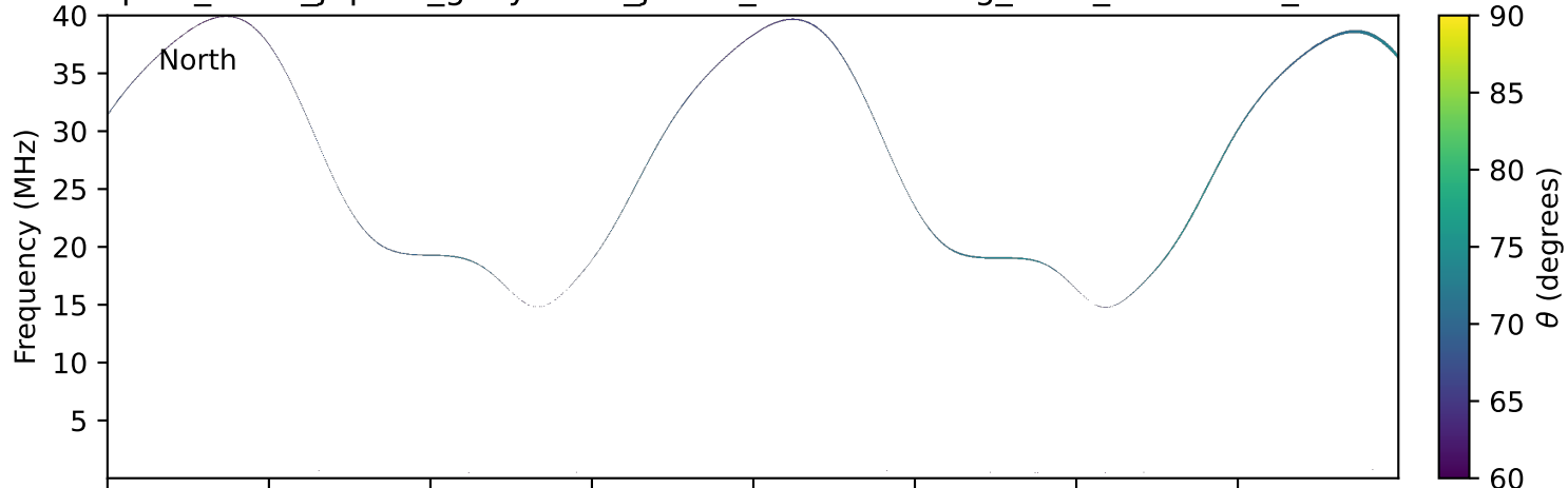
expres_earth_jupiter_ganymede_jrm33_lossc-wid1deg_3kev_20260410_v11.cdf
