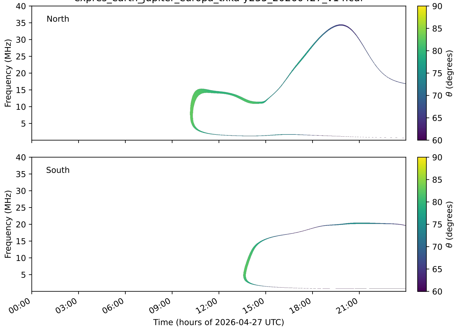
expres_earth_jupiter_europa_txka-y235_20260427_v14.cdf
