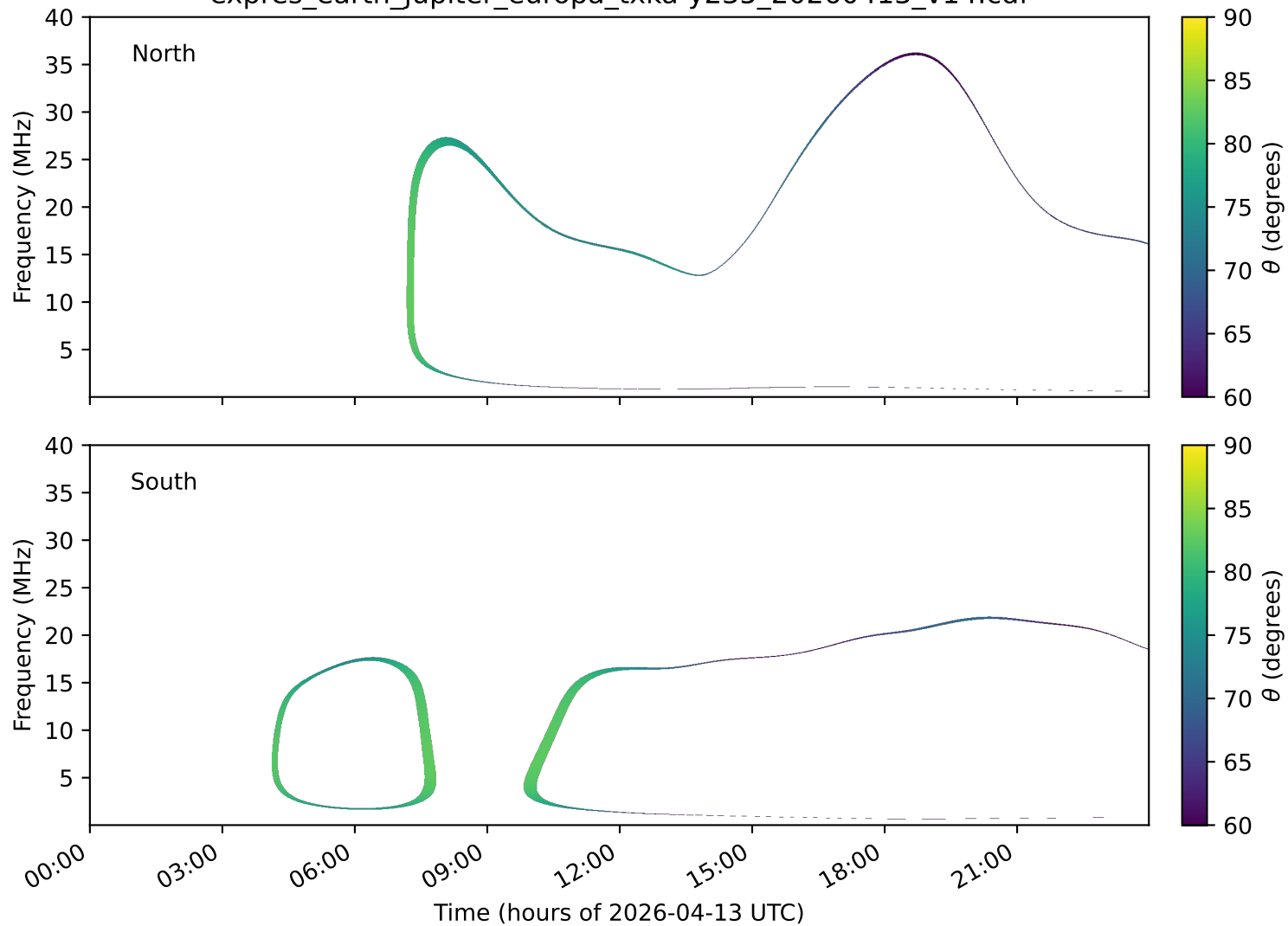
expres_earth_jupiter_europa_txka-y235_20260413_v14.cdf
